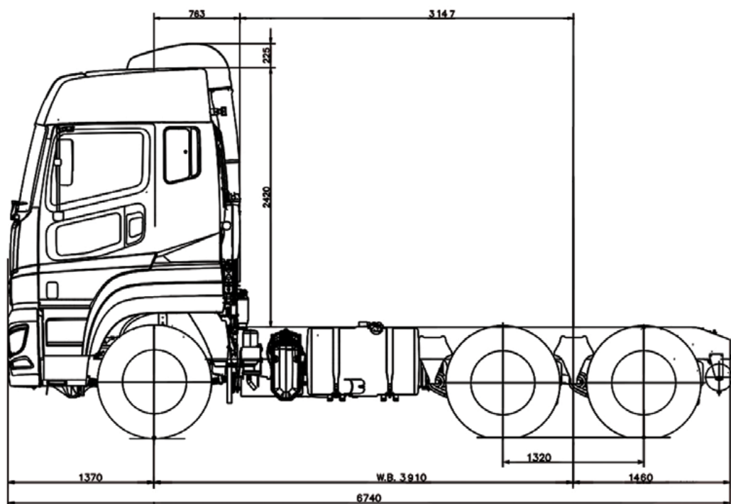
SHOGUN FV2446J 6x4 HI TOP – 'J' WHEELBASE
