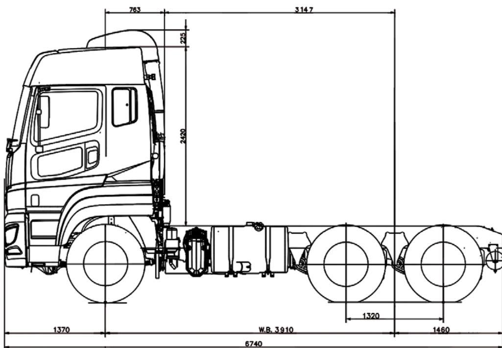
SHOGUN FV2446 6x4 HI TOP – ‘J’ WHEELBASE
